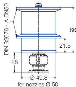
Tri-Clamp
