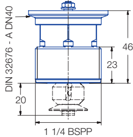
Male thread
