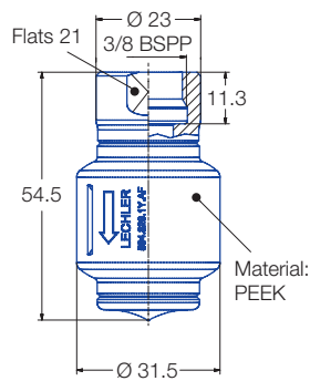
Standard version female tread 594.XX9.1Y.AF
