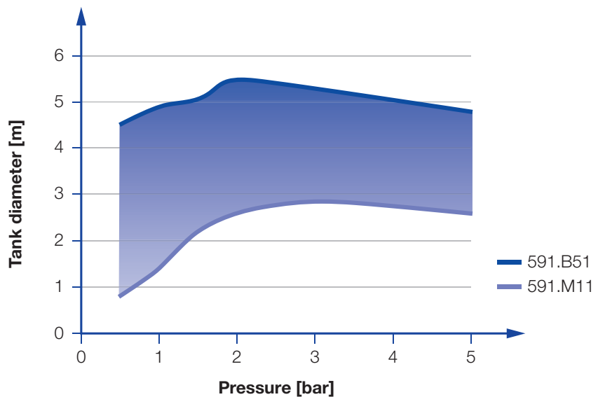
Overview of the tank diameter, depending upon the pressure of series 591
