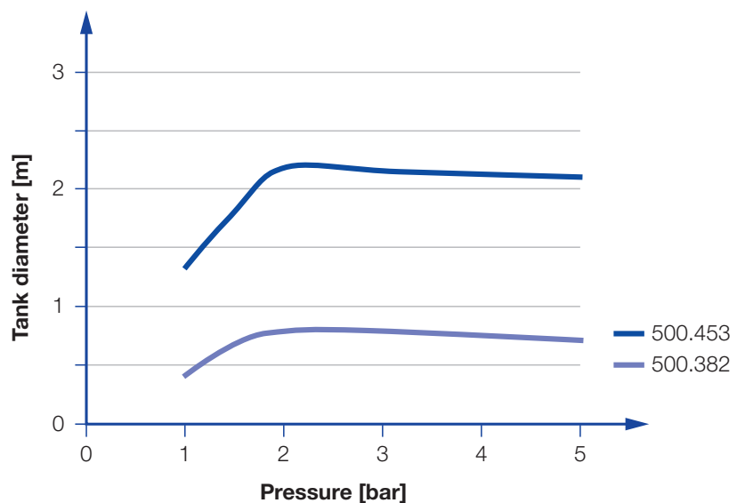
Overview of the tank diameter, depending upon the pressure of series 500.382 / 500.453
