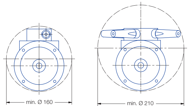
5TM.2XX.1Y.AS (2 nozzles)
