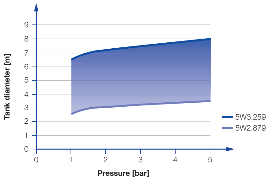
Overview of the tank diameter, depending upon the pressure of series 5W2 / 5W3
