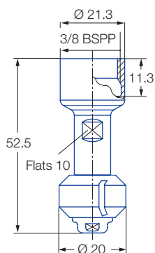
3/8 BSPP female thread
