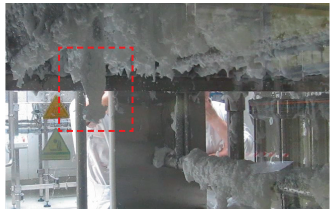
Figure 8: Foam cleaning with a Lechler PVDF MicroWhirly
