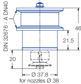
Tri-Clamp
