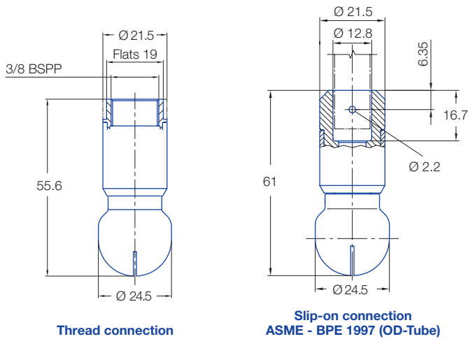
Thread connection
